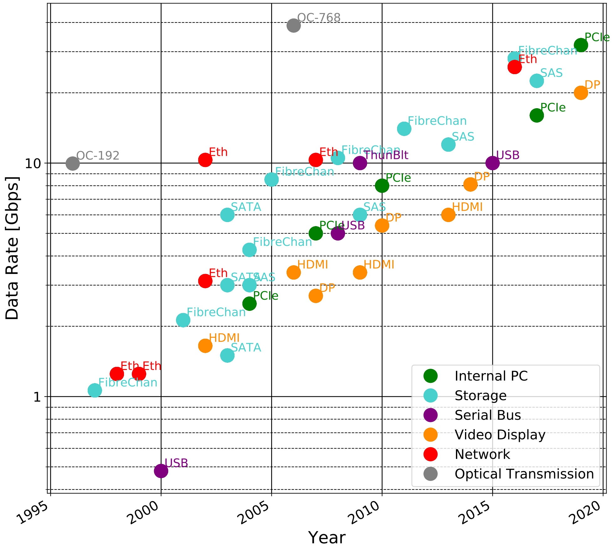
Serial Standard Line Rate vs Year
